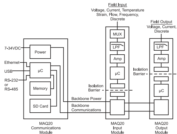
MAQ20 System Block Diagram
