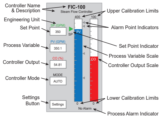
PID Faceplate in ReDAQ Shape Software
