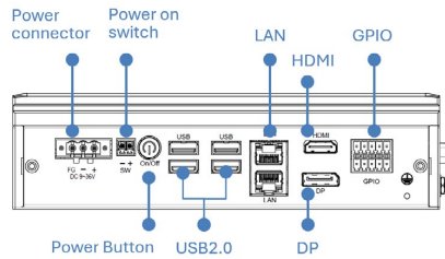
Front I/O
