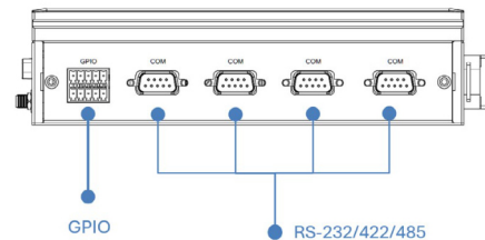
Rear I/O (with extension card)
